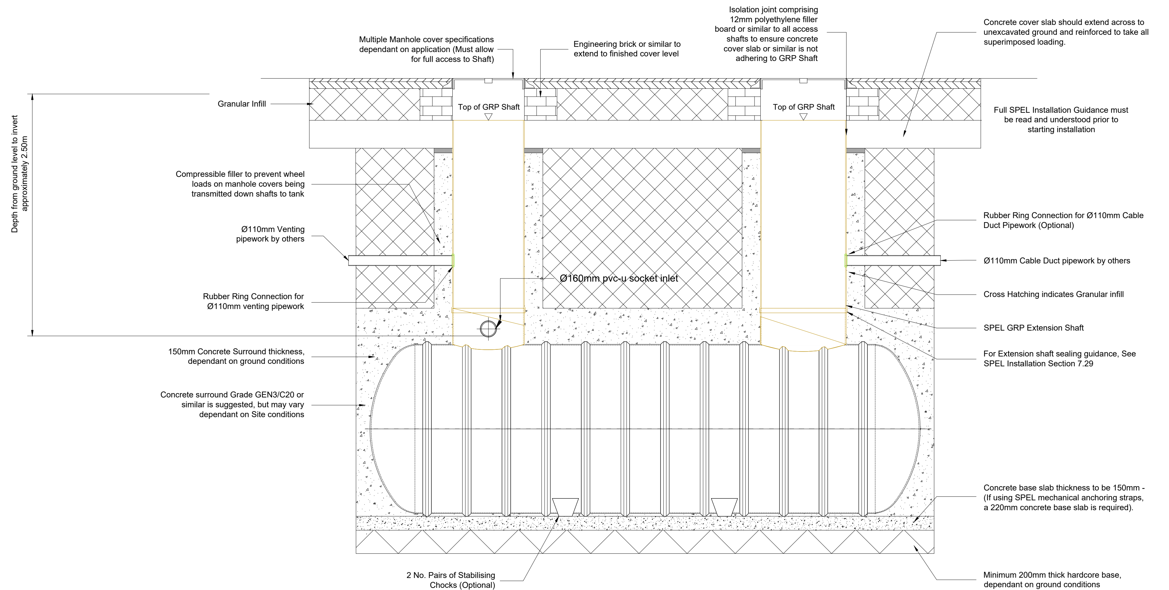
TYPICAL WASTEWATER STORAGE TANK CROSS-SECTION Scale 1:25
